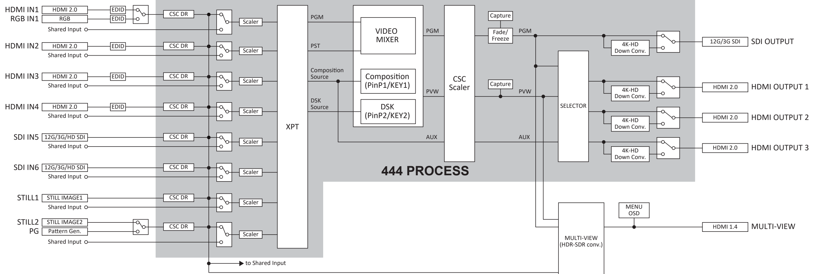
V-600UHD Ver.1.10 Video Block Diagram (2019/10/16)
