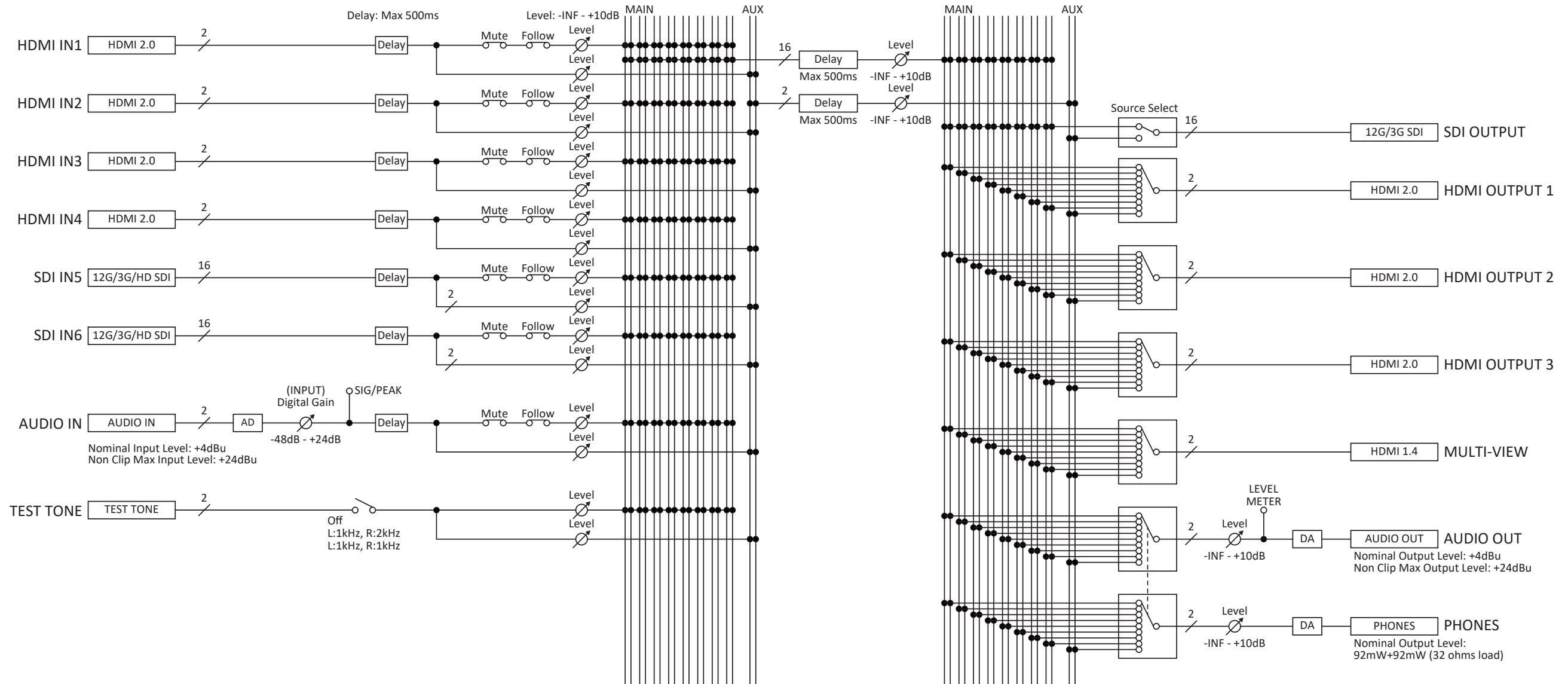
V-600UHD Ver.1.10 Audio Block Diagram (2019/10/16)
